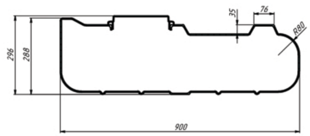
CROSS-SECTION A-A
